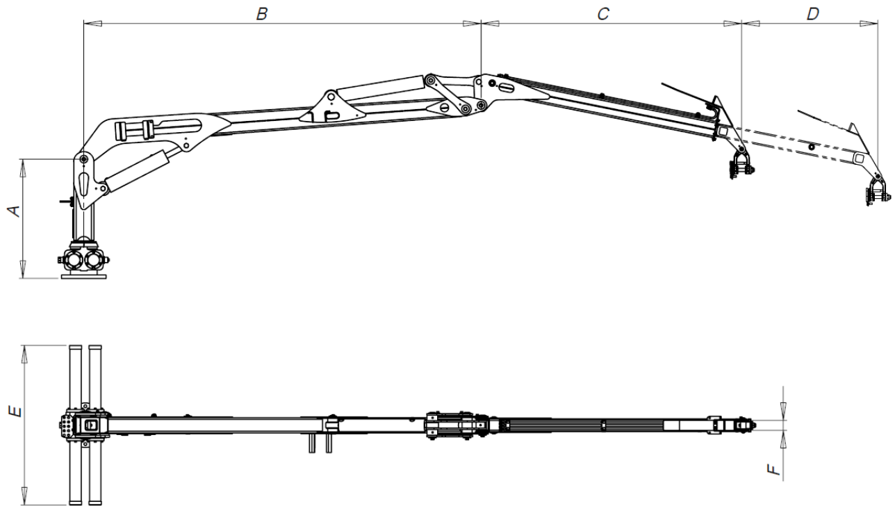
Picture: Boom system with telescopic boom extension
